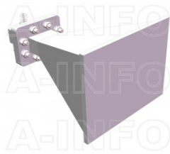
LB-159-15-C-TFSP0 Standard Gain Horn Antenna 4.9-7.05GHz 15dB Gain TNC Female
