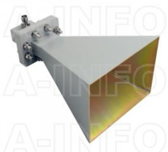
LB-159-15-C-TF Standard Gain Horn Antenna 4.9-7.05GHz 15dB Gain TNC Female
