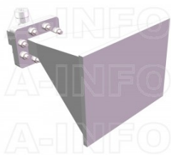
LB-159-15-C-7SPO Standard Gain Horn Antenna 4.9-7.05GHz 15dB Gain 7mm
