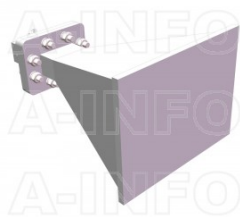
LB-159-15-C-3.5FSP0 Standard Gain Horn Antenna 4.9-7.05GHz 15dB Gain 3.5mm Female
